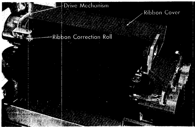
Figure 17. Ribbon Mechanism
