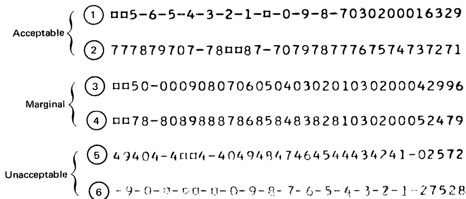
Figure 25. Ribbon Life Related to OCR Print Quality
