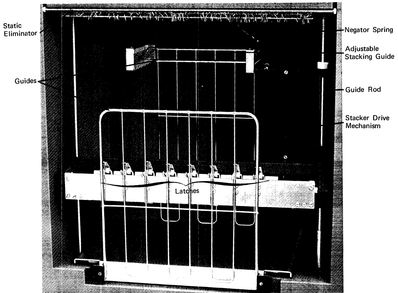
Figure 22. Forms Stacker, Model N1
