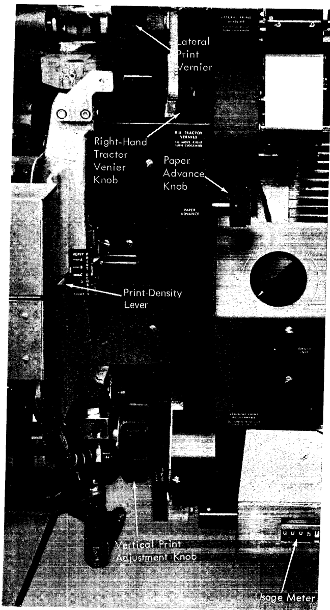
Figure 9. Manual Controls, Models 1, 2, 4, 5, 6, 7
