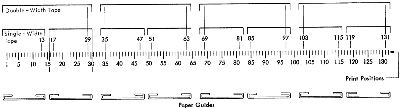
Figure 42. Print-Position Assignment
