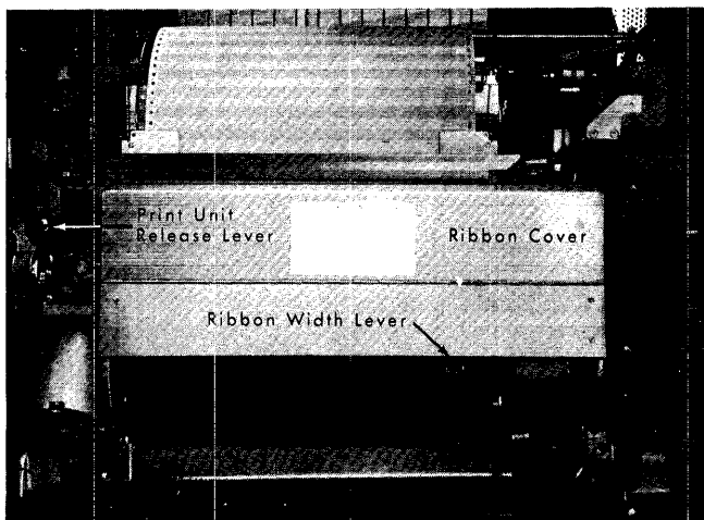
Figure 18. Front of Printer (Cover Raised)
