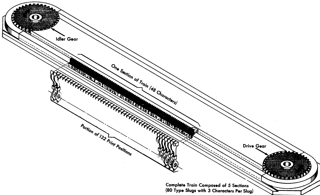
Figure 4. Schematic of Train Printing Mechanism
