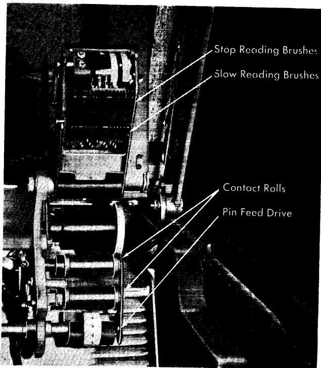
Figure 16. Carriage-Tape Brushes
